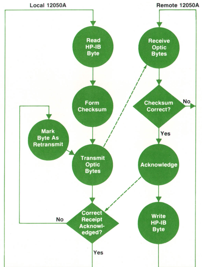
Fig. 5. Simplified flow of HP-IB data in the 12050A. Receipt of each byte is acknowledged by a handshake to the opposite 12050A.
